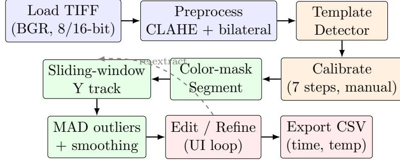
Figure 4.1: End-to-end processing pipeline. Blue stages run automatically on upload; orange stages run once per template and are persisted; green stages run on every curve request; red stages are user-driven.
